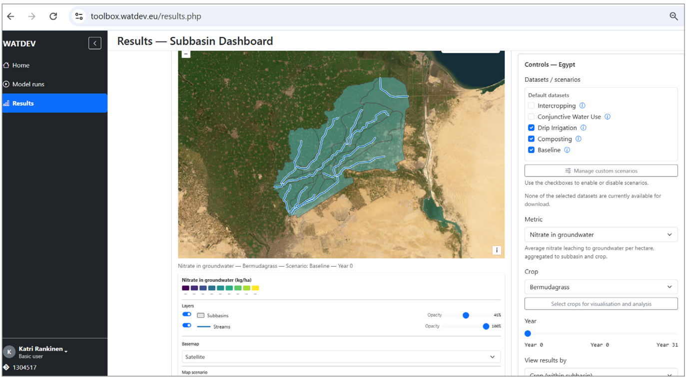
Figure 4: Subbasin dashboard
